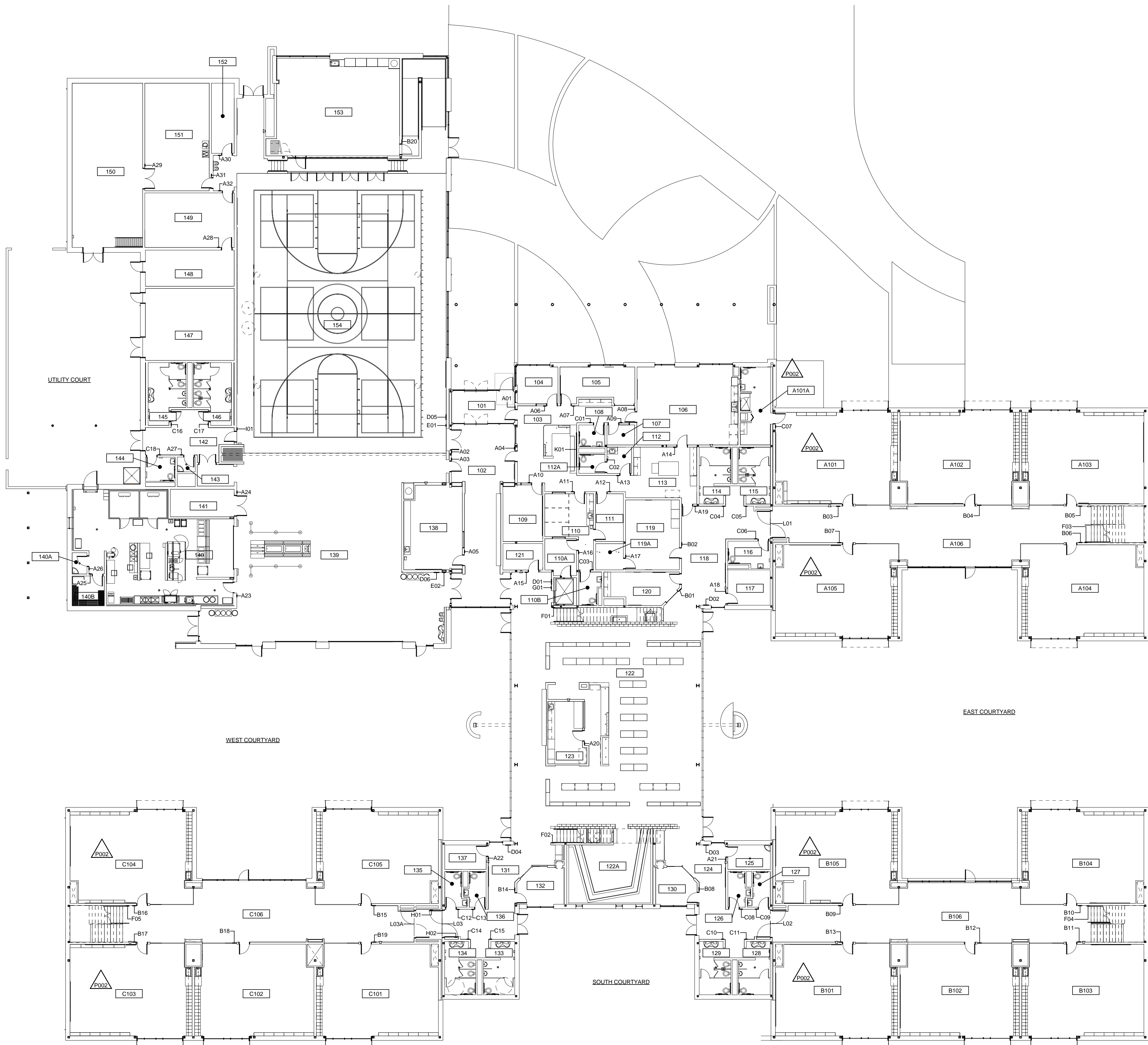
1 FIRST FLOOR SIGNAGE PLAN 1/16" = 1'-0"
