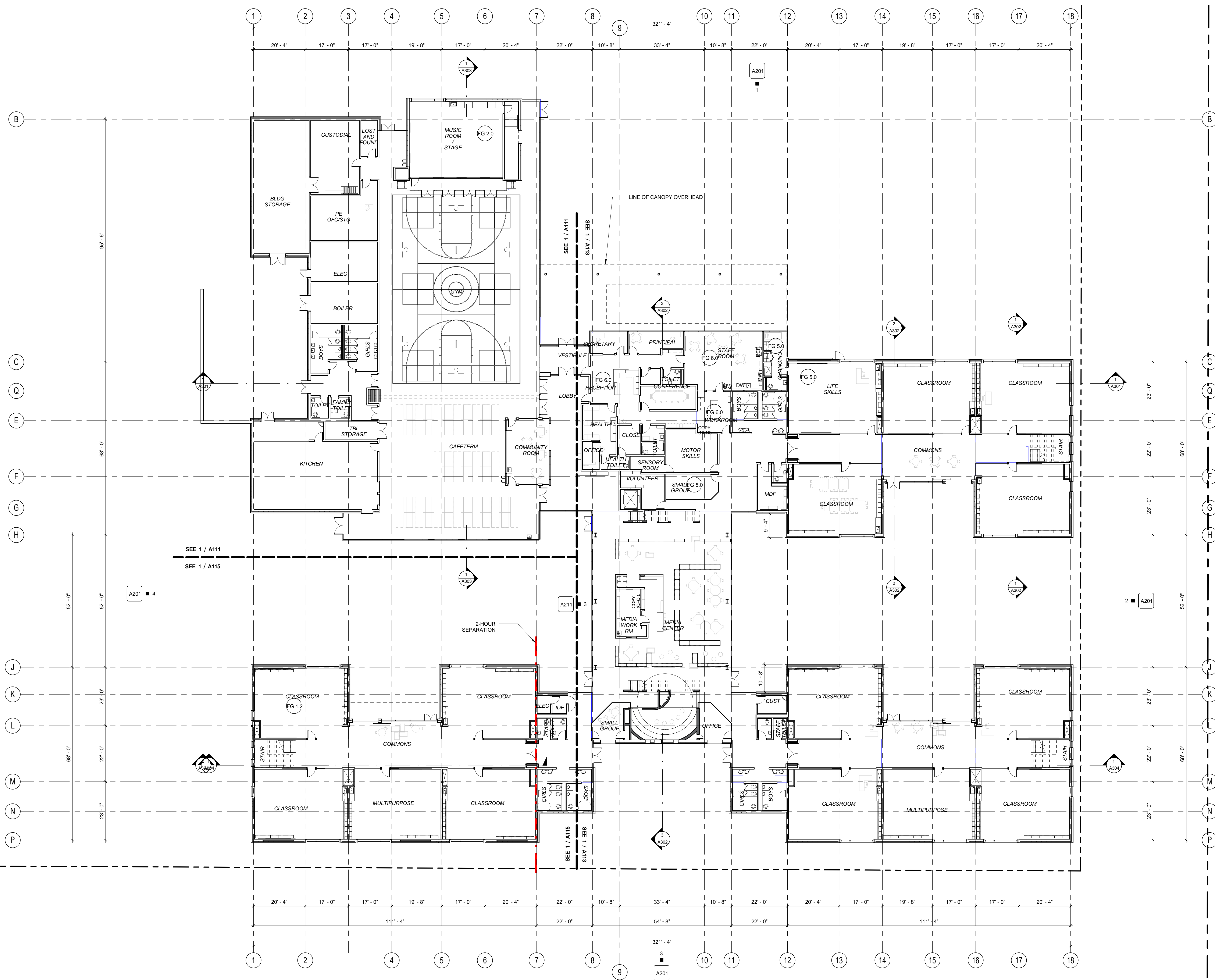
1 OVERALL FIRST FLOOR PLAN 1/16" = 1'-0"
