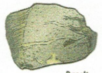
Basalt
